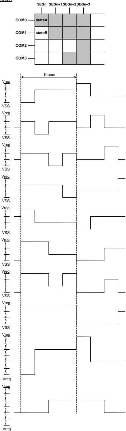
Figure 12. Waveform of Frame Inversion
